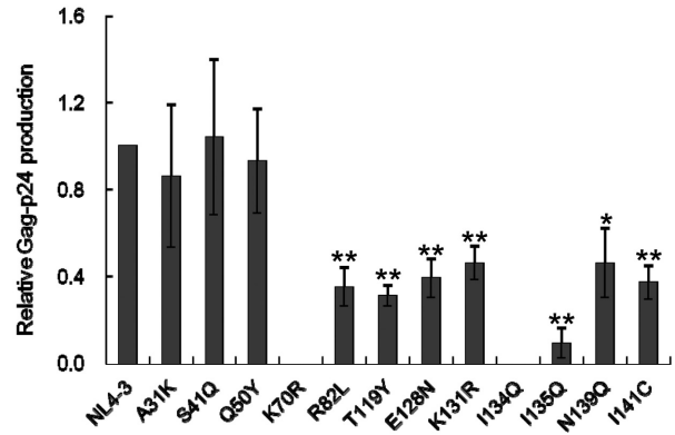
Figure 4 Ability of CA-NTD mutants derived from HIV-1 NL4-3 to produce progeny virions in H9 cells. Proviral clones indicated (2 \mu g) and pGL3 (luciferase reporter vector) (2 \mu g) were co-nucleofected into H9 cells, and on day 2 post-transfection, culture supernatants were prepared for Gag-p24 ELISA assays. Gag-p24 production by each mutant relative to that by NL4-3 is shown. Luciferase activity in cell lysates was used for normalization of the transfection efficiency. Mean values \pm SD from at least three independent experiments are presented. Significance relative to NL4-3 was determined by the Student t test (**, p < 0.01 ; *, p < 0.05 ).
