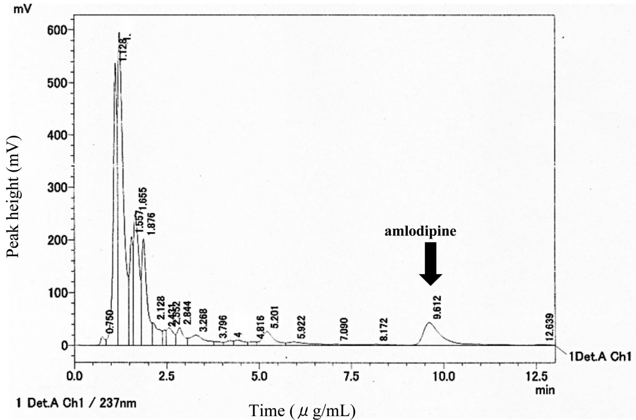
Figure 2. Typical chromatogram of the Amlodin ® + Rikkunshito suspension.
