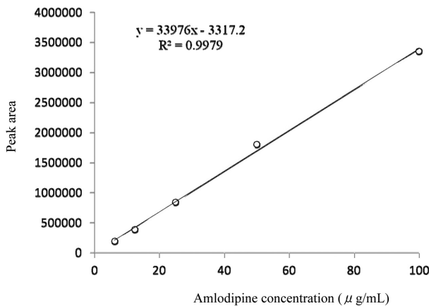
Figure 3. Calibration curve of amlodipine.
