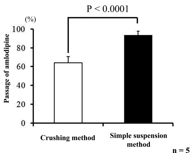
Figure 5. Comparison of the passage amounts of amlodipine between the crushing method and simple suspension method.
